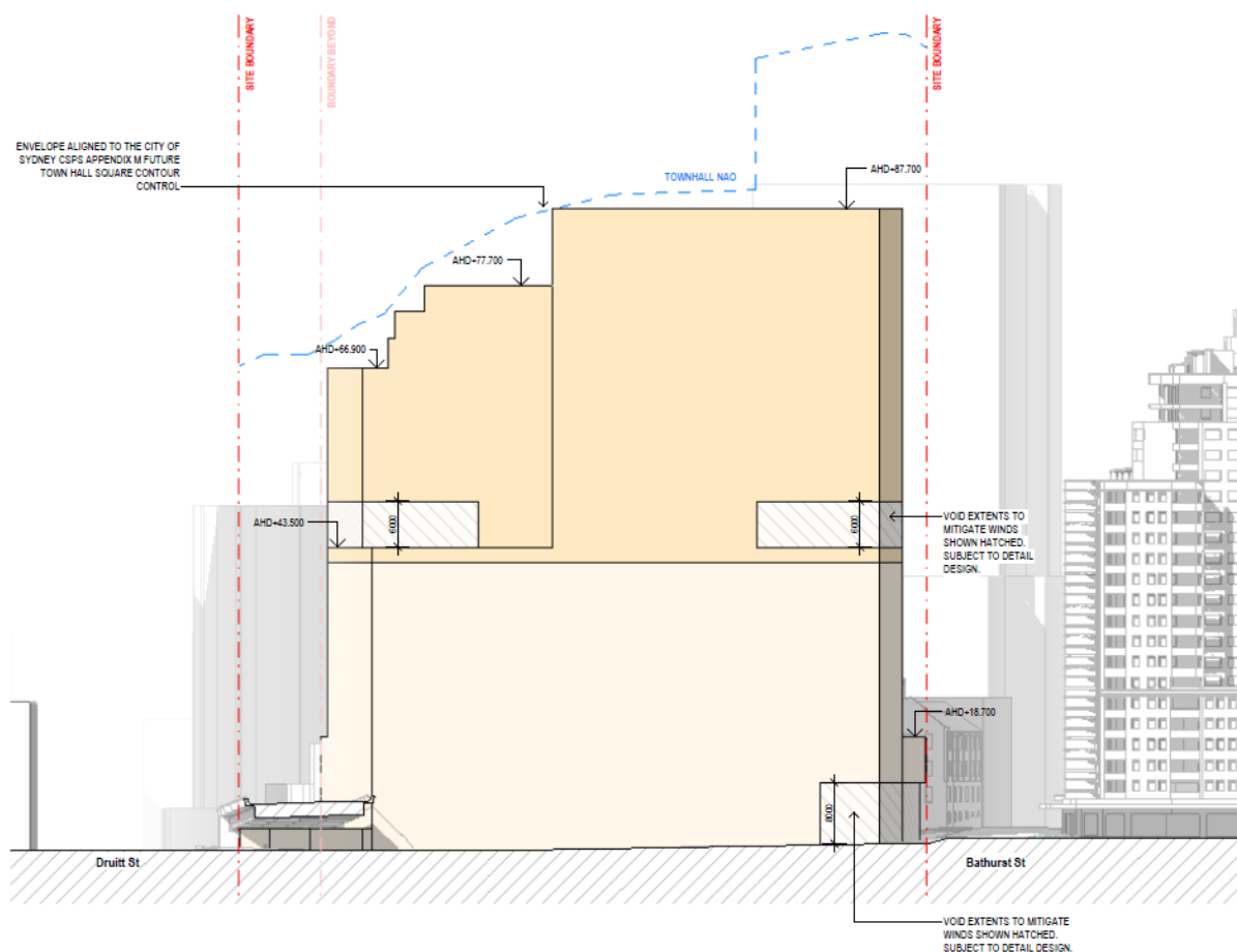
Figure 17 West elevation
